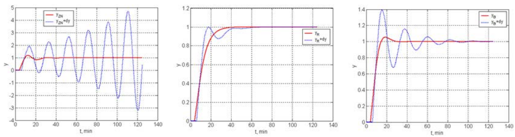
Fig. 8. The response of the control system at the step excitation for case 7
