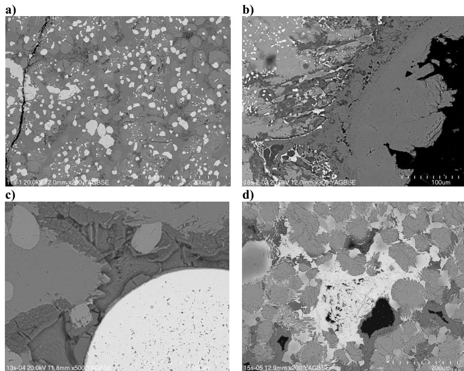
Fig. 2. Forms of metallic precipitates in the open-hearth furnace slag (white areas): a, b – fine precipitates surrounding by the glass; c – a single drop of metal; d – an irregularly shaped aggregate
