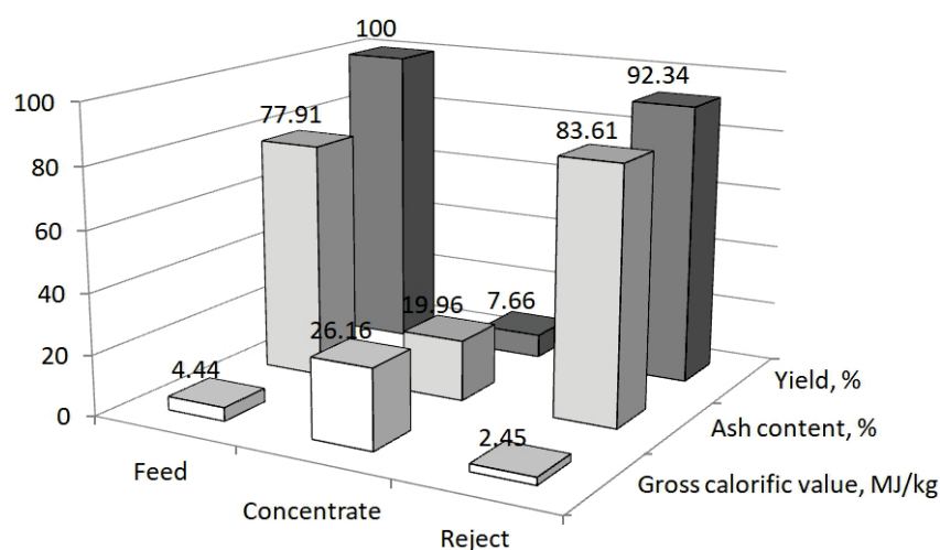
Fig. 3. The parameters of feed and the products of washing – industrial tests (Róžański et al. 2016)
