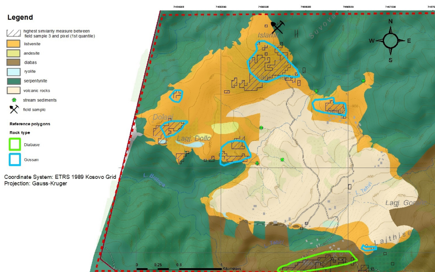
Fig. 8. Comparison of the similarity coefficient between rock sample 3 and the satellite image. The geological map used as a background
