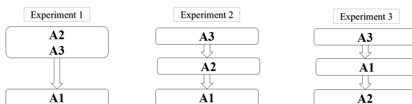
Fig. 4. Final rankings of three computational experiments (developed by the author)
