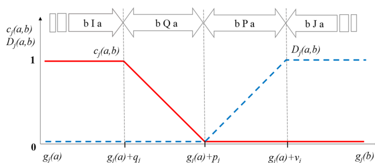
Fig. 2. The model of four preference situations (indifference I , weak preference Q , strict preference P , incomparability J ) based on threshold values q_j , p_j i v_j (based on Zak and Sawicki 1999)
