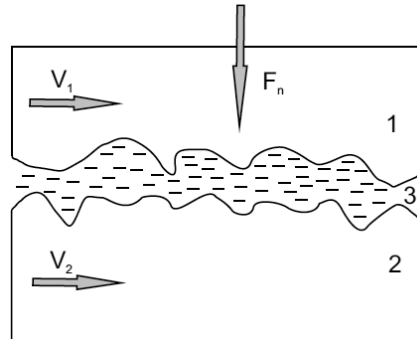
Fig. 1. Diagram of the tribological system 1 – an element exciting relative motion, 2 – an element taking over the kinematic excitation, 3 – intermediating layer, F_n – load, V_1 , V_2 – velocities of the elements of the tribological pair
