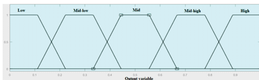
Fig. 2. Membership functions of output variable
