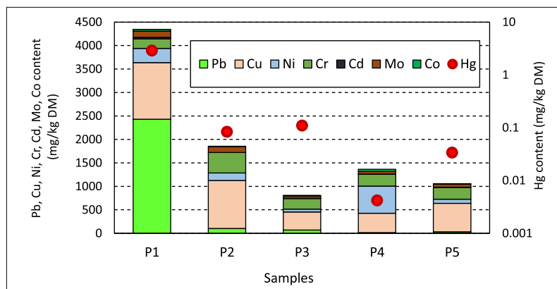
Fig. 1. Heavy metals content in the tested dusts (the mean of obtained results)
