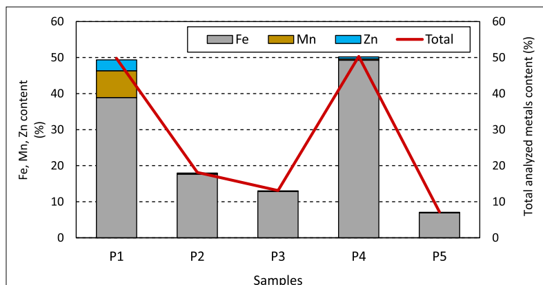
Fig. 2. Fe, Mn, Zn content in tested dusts (the mean of obtained results)
