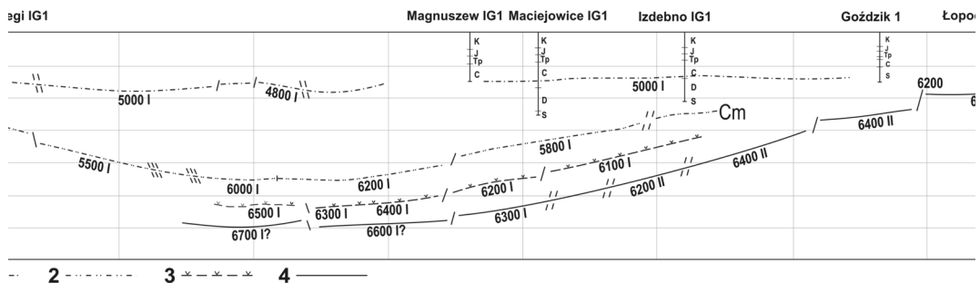
Fig. 4. Interpretation of the refractive seismic study results in the Białobrzegi–Goździk section (1–X/VI–63/71); 1 – boundary traced within the Palaeozoic; 2 – boundary associated with the Cambrian; 3 – boundary associated with younger ground; 4 – boundary associated with older ground
