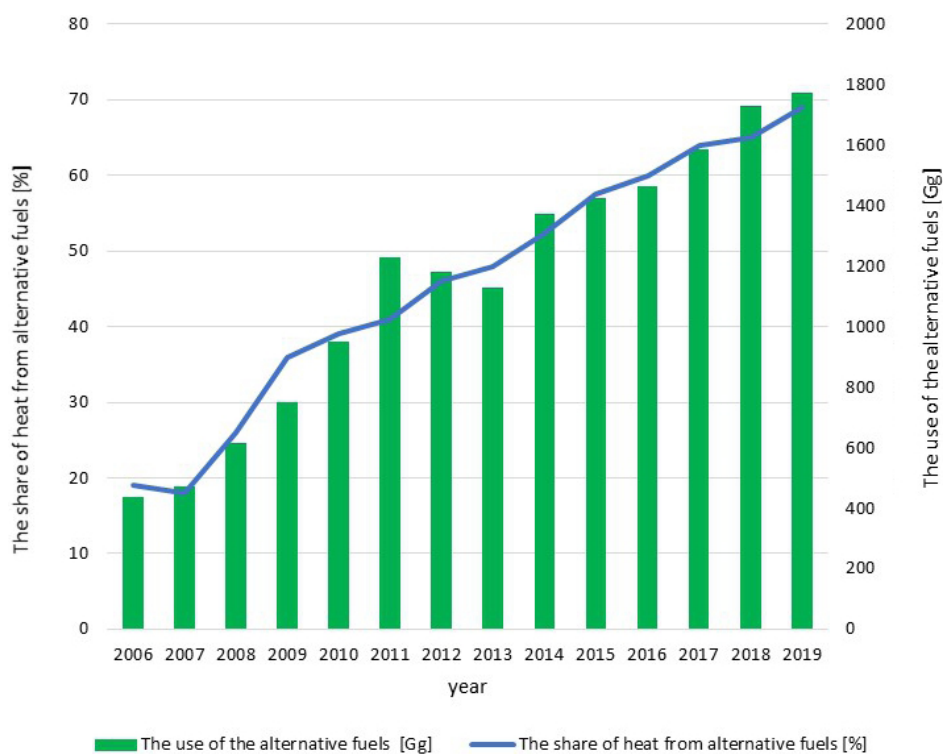
Fig. 2. The use of the alternative fuels in the cement industry (2006–2019), based on the data from PCA 2010–2022 and Uliasz-Bocheńczyk et al. 2021
