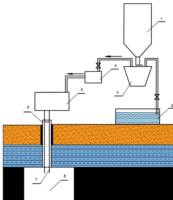
Fig. 2. Liquidation of the void in the rock mass by injection of ash-water mixture according to (Kubański 2008)
