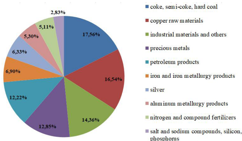
Fig. 2. Volume of Polish mineral resources exports in 2020 (PGI-NRI 2022)
