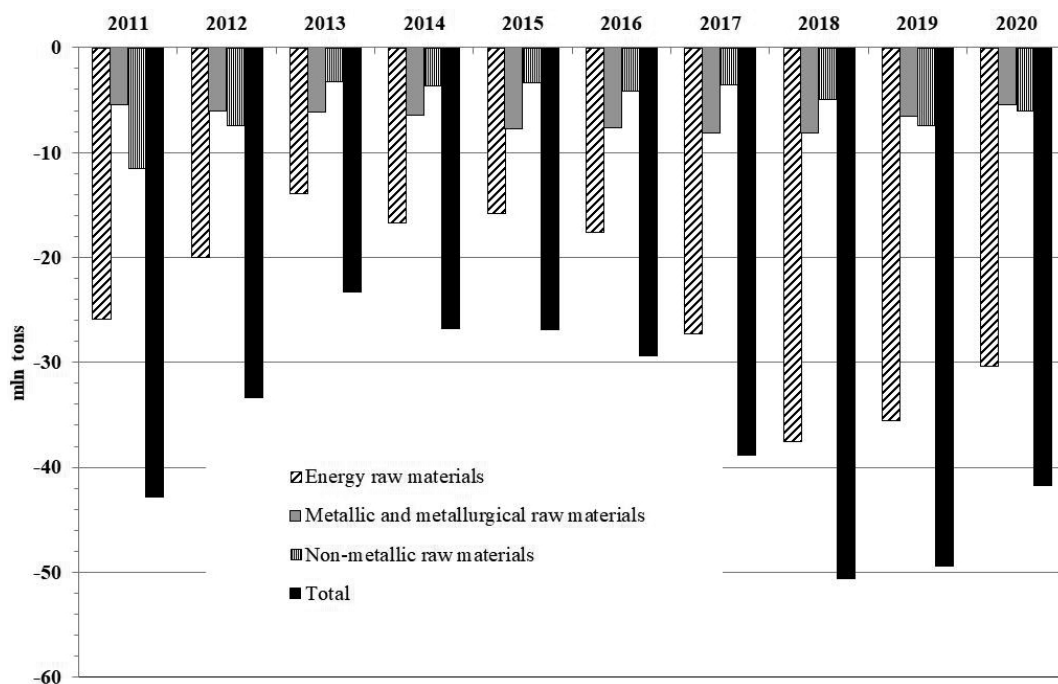
Fig. 3. The quantitative balance of trade in mineral resources in Poland (according to PIG-PIB 2021 )
