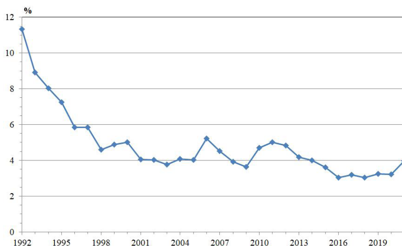
Fig. 1. The share of exports of metallic raw materials in Poland in relation to all exported goods (WORLD BANK 2022)
