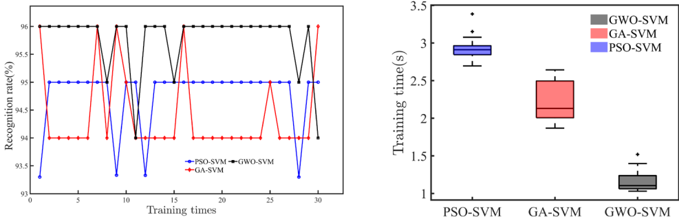
Fig. 13. Algorithm classification results a) Model classification rate, b) Model classification time Source: own study
