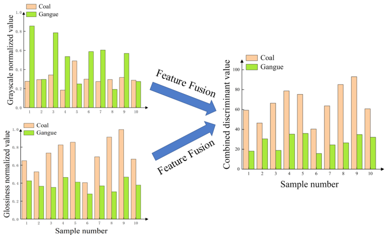
Fig. 9. Feature tandem fusion
