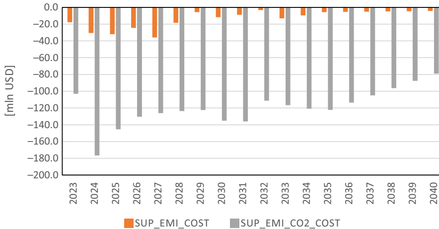
Fig. 10. Comparison of CO 2 Emission Allowances costs for centrally dispatched power generation units under the analyzed research scenarios – difference related to the SUP_COST scenario (mln USD) Source: own study
