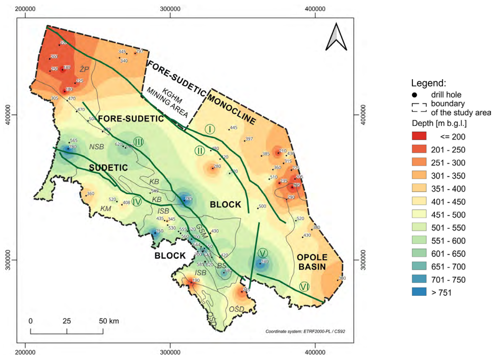
Fig. 3. Depths at which 20°C was measured; explanation of tectonic units as in Figure 1
