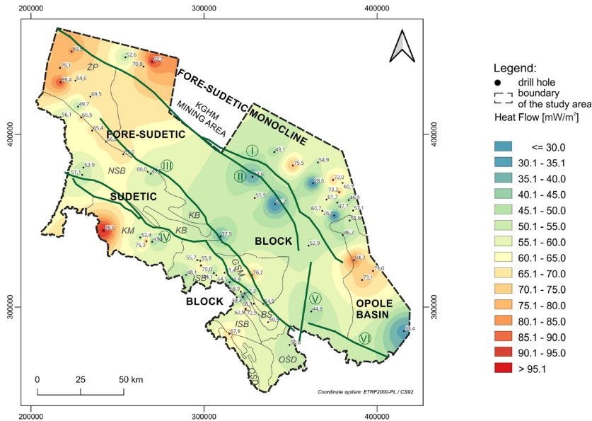
Fig. 7. Heat flux density variation; explanation of tectonic units as in Figure 1
