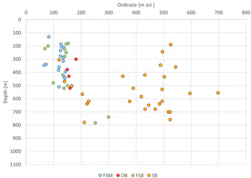
Fig. 4. Depths at which temperatures of 20°C were measured versus the height of the boreholes above sea level FSM – Fore-Sudetic Monocline, FSB – Fore-Sudetic Block, OB – Opole Basin; SB – Sudetic Block
