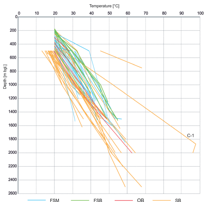
Fig. 2. Results of thermal logs in the analysed boreholes FSM – Fore-Sudetic Monocline, FSB – Fore-Sudetic Block, OB – Opole Basin; SB – Sudetic Block
