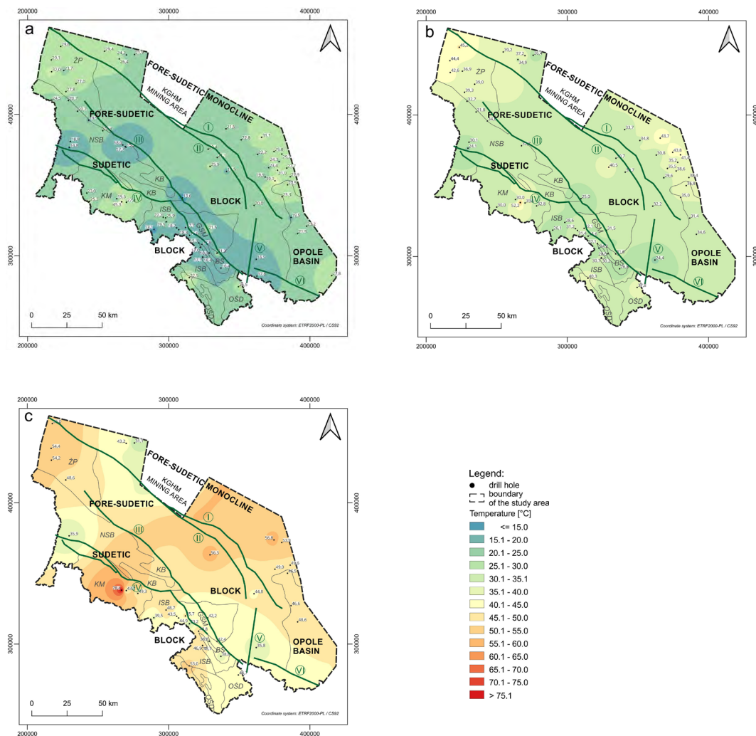
Fig. 6. Spatial temperature distribution at depths
