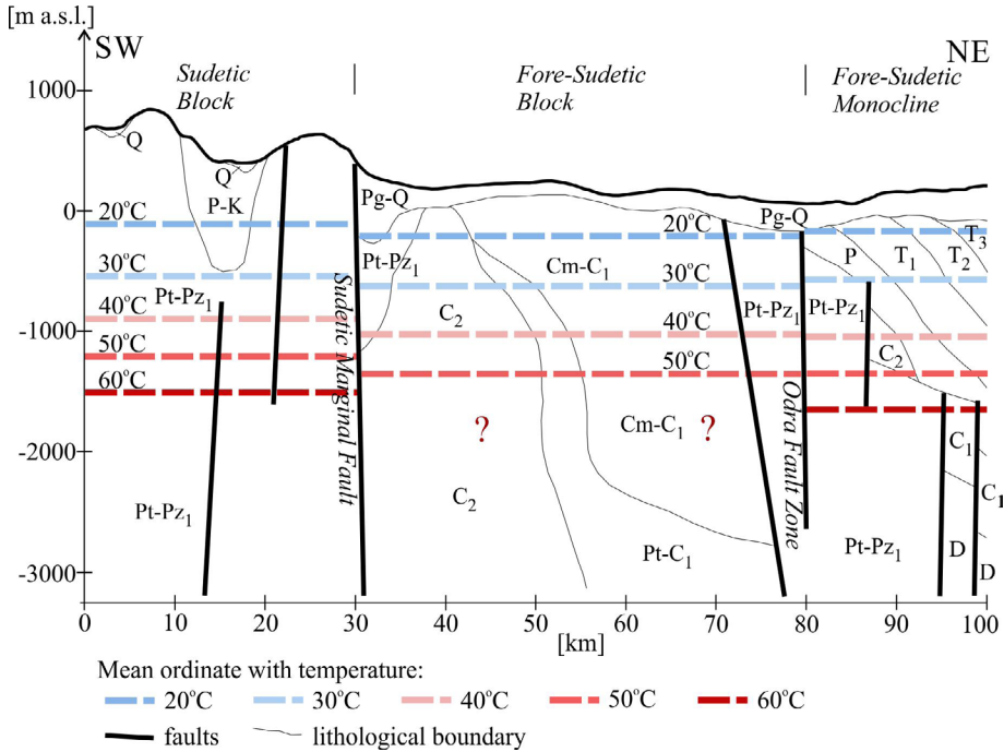
Fig. 8. Diagram of the temperature distribution in the study area (geological structure according to https://geologia.pgi.gov.pl/mapy )
