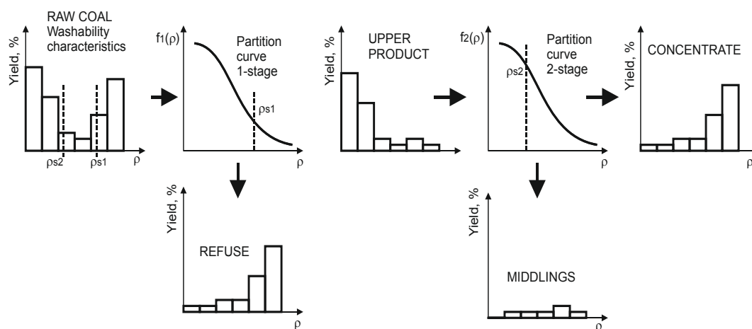
Fig. 3. A model of the three-product coal separation process in a jig
