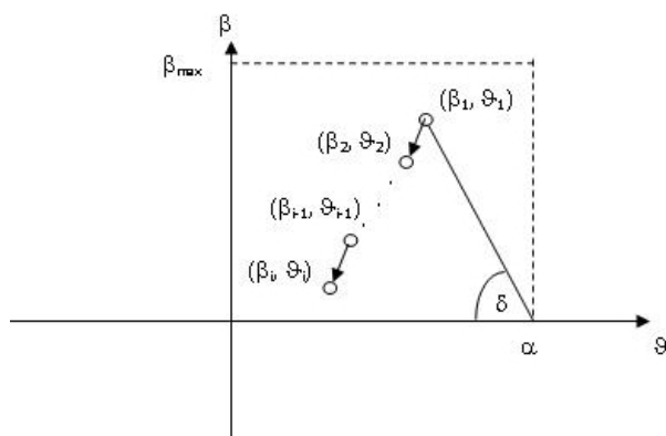
Fig. 1. Elements of the analysis of ore upgradeability, where tg\delta = \frac{\gamma}{100} - 1 , \beta_{max} is the useful component content in its richest mineral, \alpha = const , \gamma = \frac{\alpha - \vartheta}{\beta - \vartheta} \cdot 100\%
