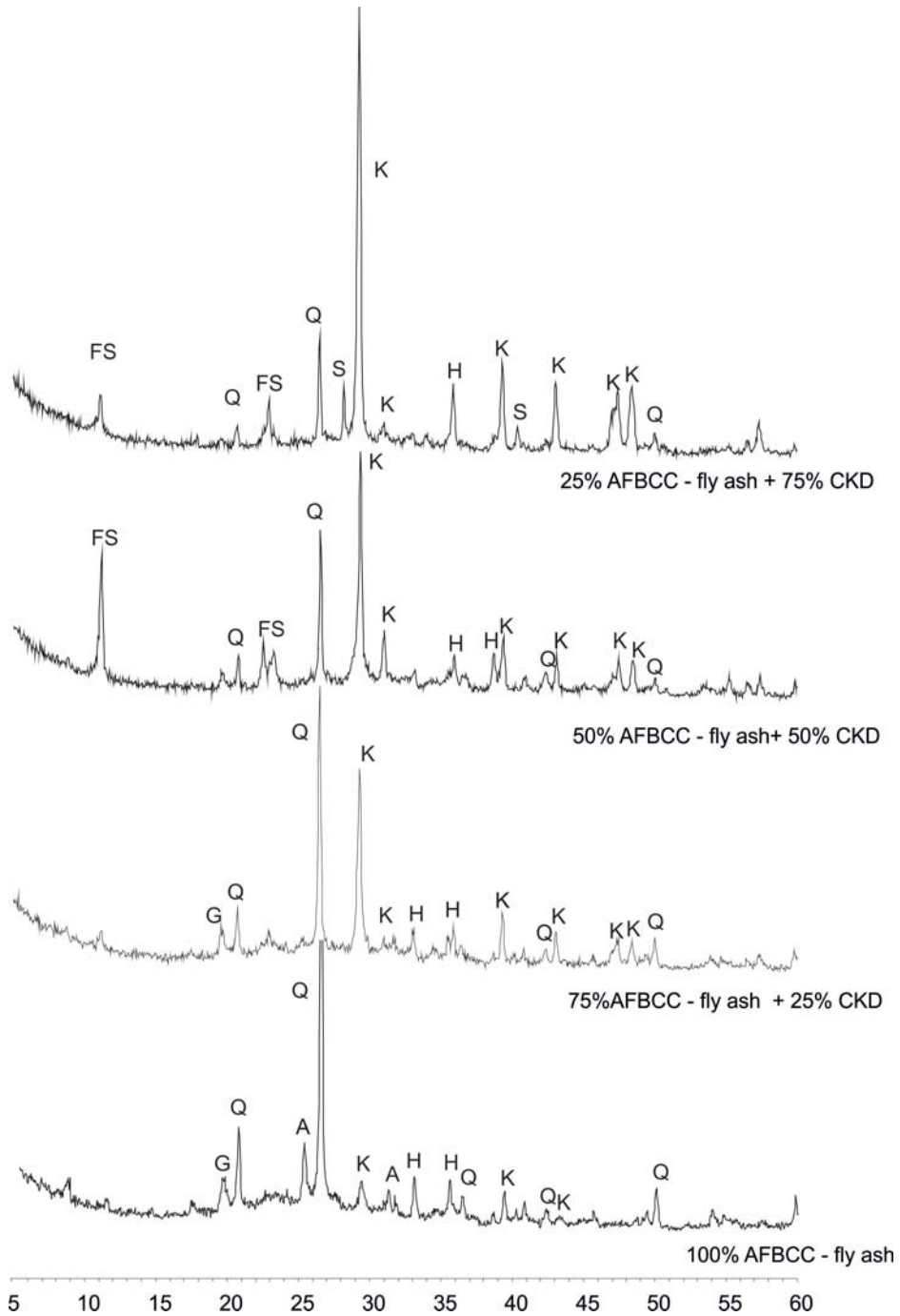
Fig. 3. Diffractograms of grouts used for the research
