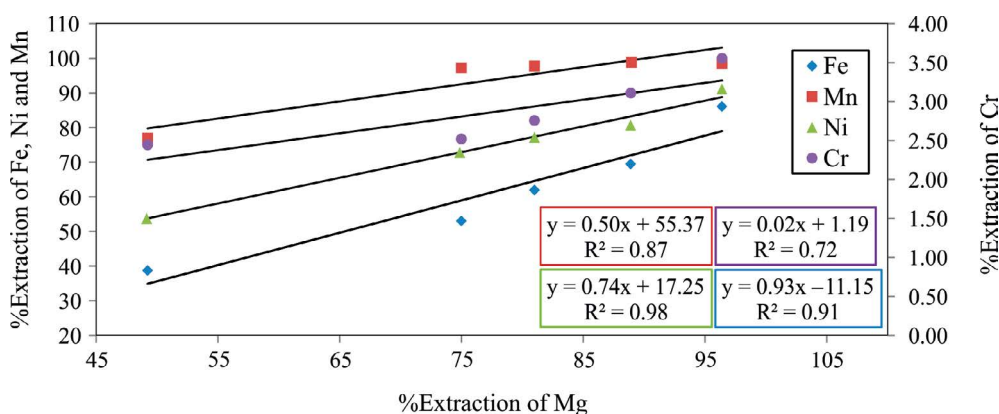
Fig. 7. Extraction correlation for magnesium, iron, chromium and nickel in the HCl leaching (Extraction values were taken from Fig. 6c)
