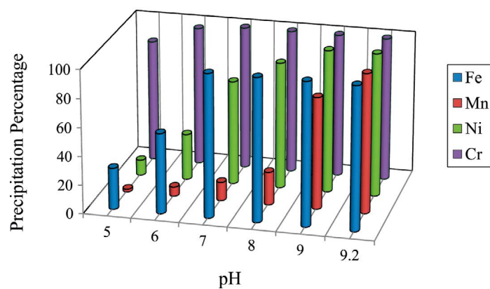
Fig. 10. Precipitation percentage of the impurities by pH
