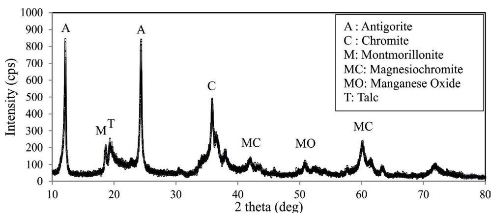
Fig. 2. XRD pattern of the fine sized tailings
