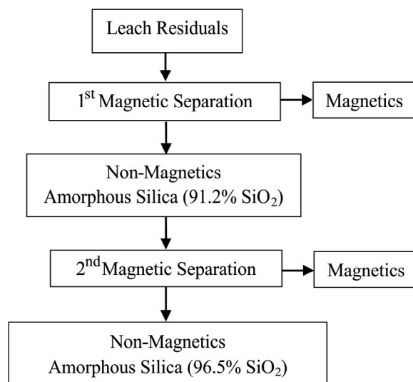
Fig. 9. Flow chart of the additional magnetic separations
