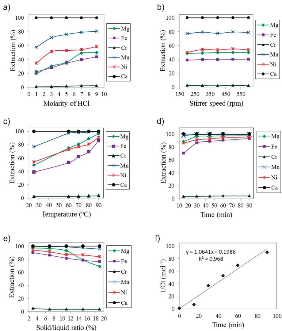
Fig. 6. a) Effects of HCl concentration (solid/liquid rate: 7%; stirring time: 30 min; stirrer speed: 300 rpm, temperature: 25°C), b) stirrer speed (solid/liquid rate: 7%; stirring time: 30 min; HCl concentration: 7 M, temperature: 25°C), c) temperature (solid/liquid rate: 7%; stirring time: 30 min; stirrer speed: 300 rpm; HCl concentration: 7 M), d) time (solid/liquid rate: 7%; stirrer speed: 300 rpm; temperature: 90°C; HCl concentration: 7 M), e) solid/liquid rate (stirrer speed: 300 rpm; stirring time: 30 min; temperature: 90°C; HCl concentration: 7 M) on leaching and f) the second order dissolution kinetics of magnesium
