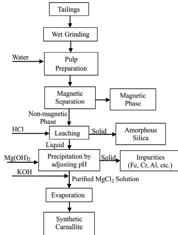
Fig. 4. Basic flow sheet of the experimental study
