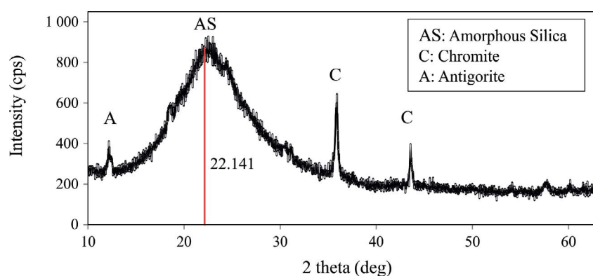
Fig. 8. XRD Pattern of the leach residual
