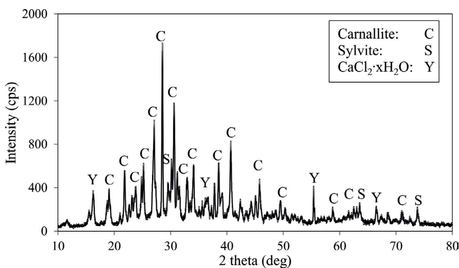
Fig. 12. XRD pattern of the synthesized carnallite
