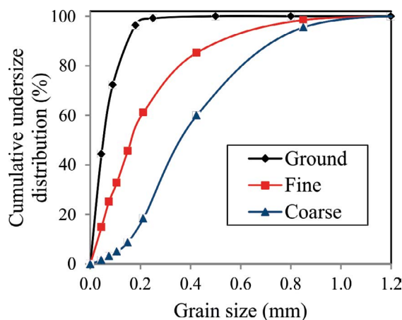
Fig. 3. Cumulative undersize distribution of the fine, coarse and ground tailings
